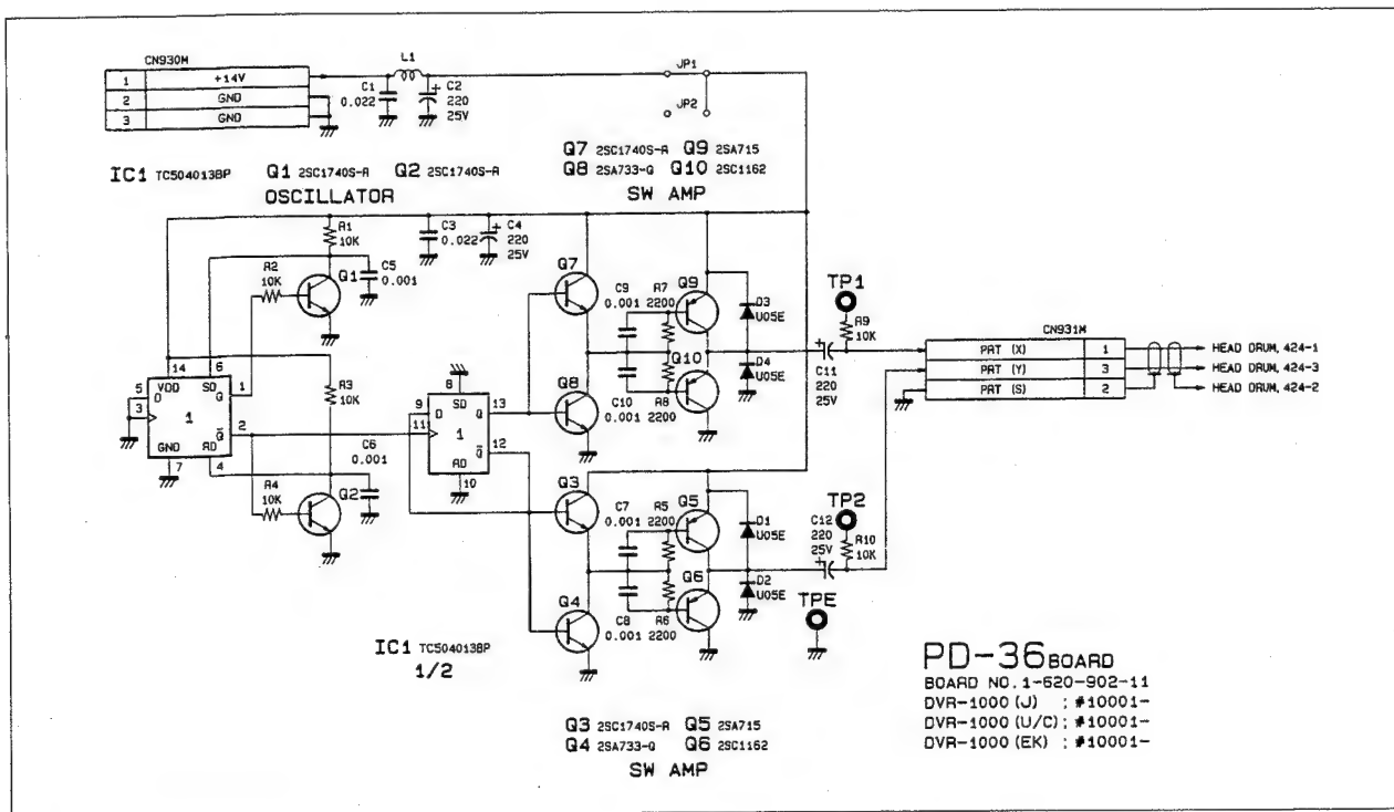
Fig. 4-7-1. PD-36 board
